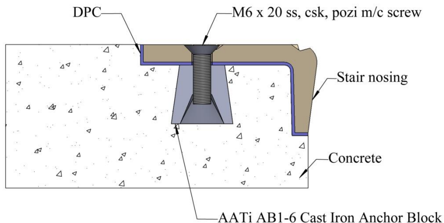
Fig 1. Section view of fixing detail for SN30/60
