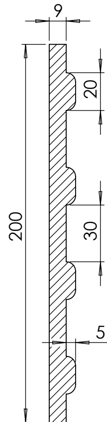
Section view scale 1:2
