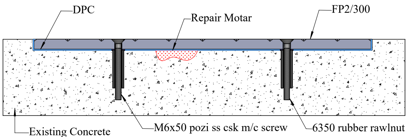
Fig 1. Section view of fixing detail
