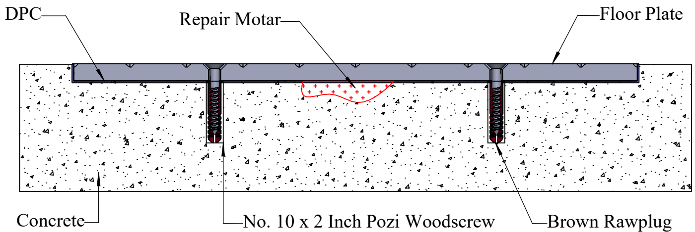
Fig 1. Section view of fixing detail
