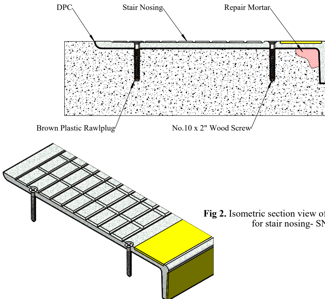
Fig 1. Section view of fixing detail for stair nosing- SN293/WL/307UR
