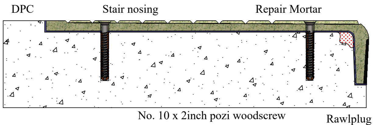
Fig 1. Section view of fixing detail for stair nosing- SN93/SL3/280
