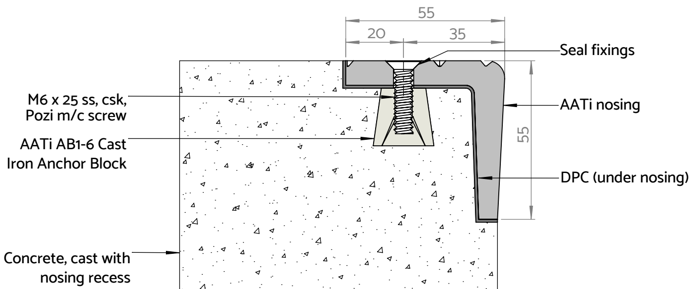
Fig 1. Sectional view of SN9/55 cast into concrete with Anchor Blocks assembly
