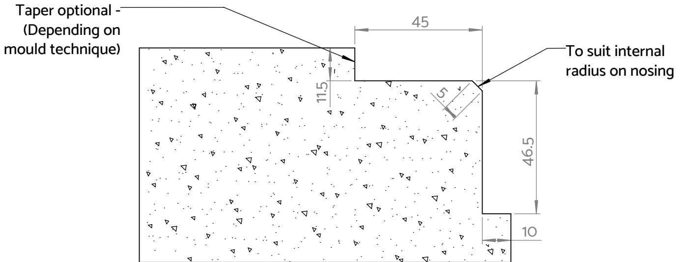
Fig 1. Sectional view of SN9/55 Recess detail
