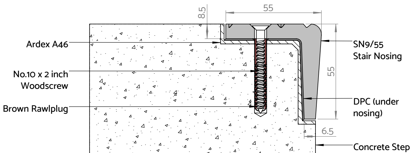
Fig 2. Sectional view of SN9/55, Recess detail assembly
